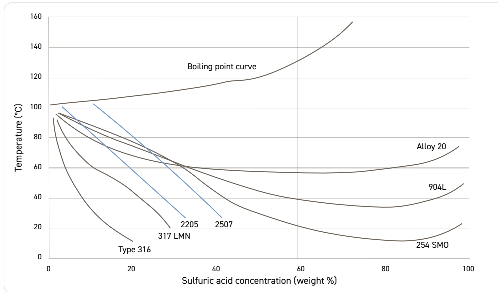
Figure 3.2 Corrosion in non-aerated sulphuric acid, 0.1 mm/yr (0.004 inch/yr) isocorrosion diagram (laboratory tests using reagent grade sulphuric acid). Source: Producer data sheets, 254 SMO is a trademark of Outokumpu.
