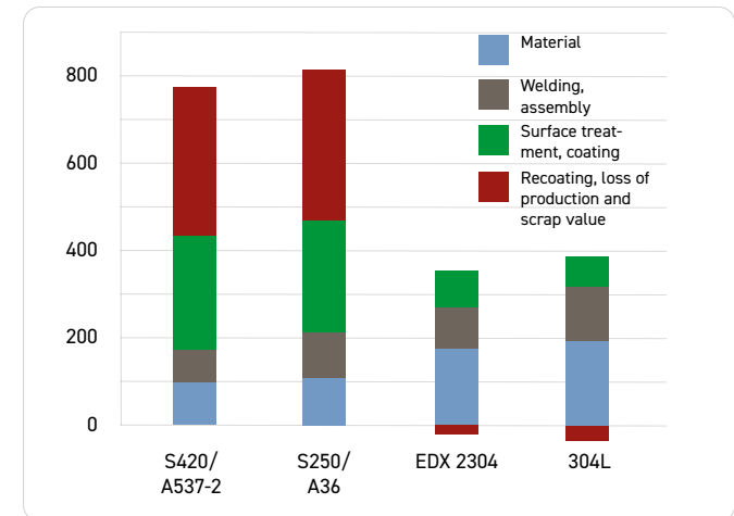
Figure 6.1 LCC of a duplex tank (Ref 6.13.6)
