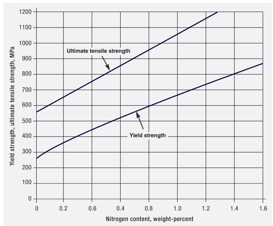
Figure 13: Effect of nitrogen on the strength of austenitic stainless steels. (9)
