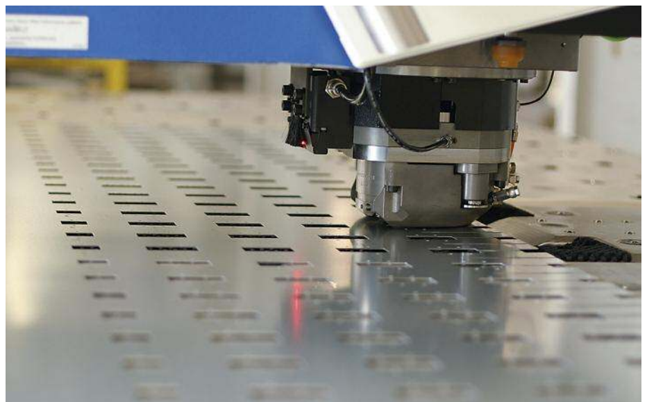
Piercing operation to produce a perforated stainless steel sheet.
