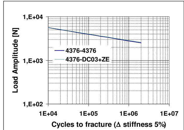
Figure 5: Comparison of fatigue tests of spot welded and spot welded + bonded samples Graph for 50% -Break down probability, R=0,1 / f=90 Hz / T=25^{\circ}\text{C}
